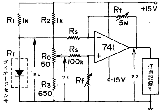
Fig. 2 Practical circuit of the temperature measurement using a diode sensor.
