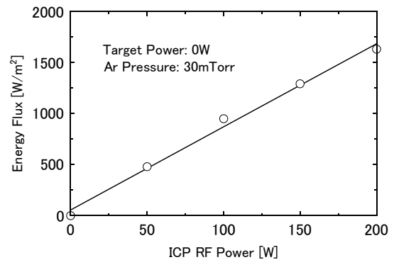
Figure 5. ICP RF power dependence of energy flux (operation with ICP alone).
