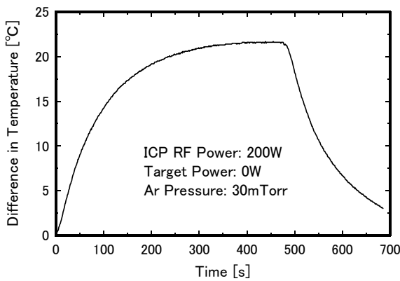
Figure 3. Temporal change in temperature difference obtained by a thermal probe during on and off period of 200W ICP.
