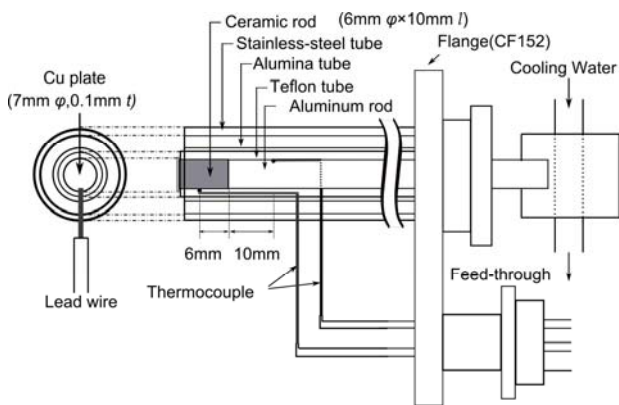
Figure 1. Schematic of thermal probe.
