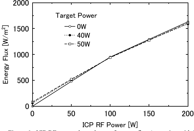
Figure 6. ICP RF power dependence of energy flux (operation with ICP assisted PM sputtering).
