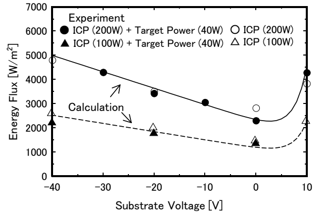
Figure 7. Substrate bias dependence of energy flux: Comparison of measured and calculated energy flux.
