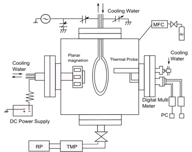
Figure 2. Experimental setup for the energy flux measurement in ICP assisted sputter-deposition.
