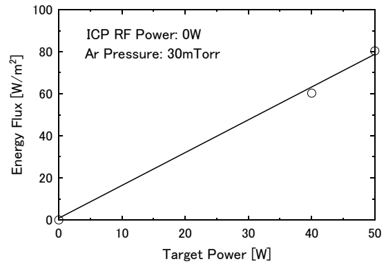
Figure 4. Target power dependence of energy flux (operation with PM alone).
