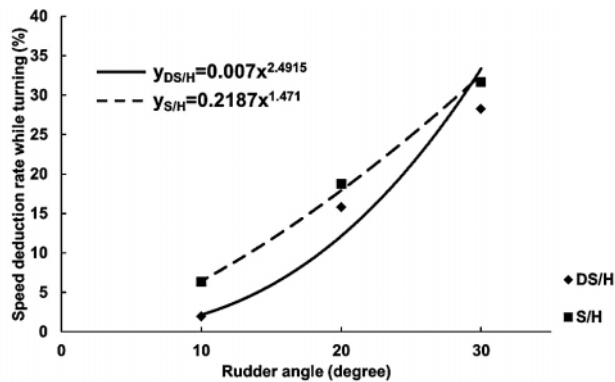
Fig.13 Speed deduction rate while turning by ship speed and rudder angle using two engines and two rudders (on 13, Nov. 2009)
