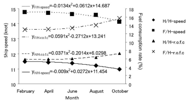
Fig. 3-1 Variations of rate of monthly ship speed and fuel consumption rate (February-October)
