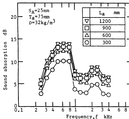
Fig. 11 Effects of the length of treatment of the duct on sound absorption
